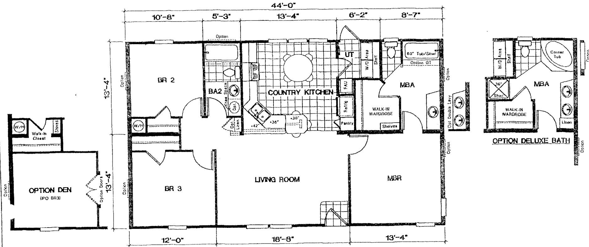
PRELIMINARY BUCKEYE MODEL 4428-XXZ / SVS SERIES THREE BEDROOM, 2 BATH, 1174 SQ. FT.
